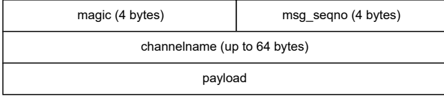
Fig. 2. LCM packet format
